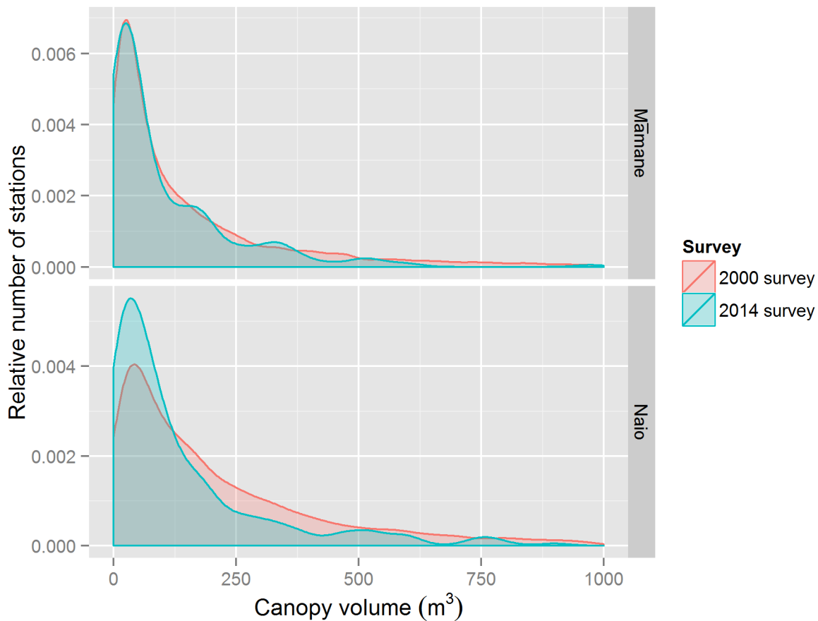
Figure 6. Distribution of tree canopy volume for māmane and naio trees in the 2000 and 2014 surveys.
