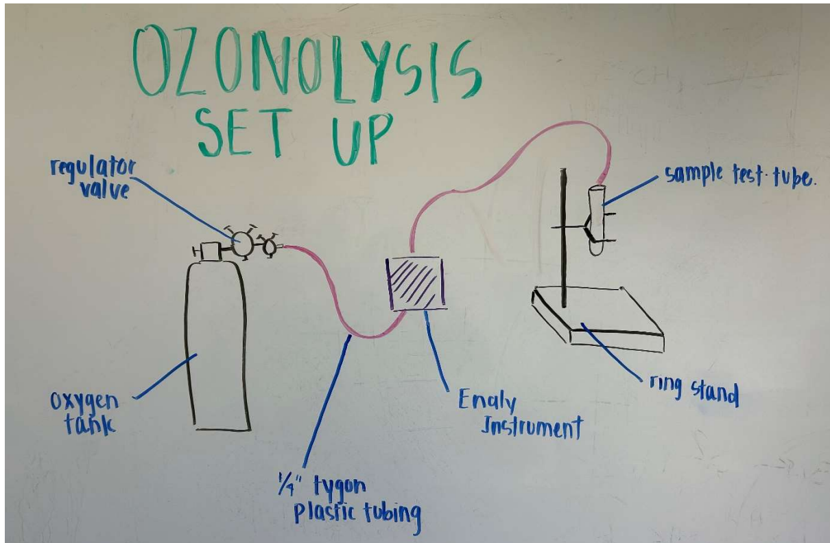
Figure a1: Ozonolysis set-up diagram consisting of oxygen tank, regulator valve, 1/4' tygon plastic tubing, Enaly instrument (ozone generator), ring stand and sample test-tube.
